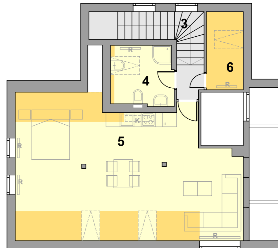
Mansarda M 1:100
