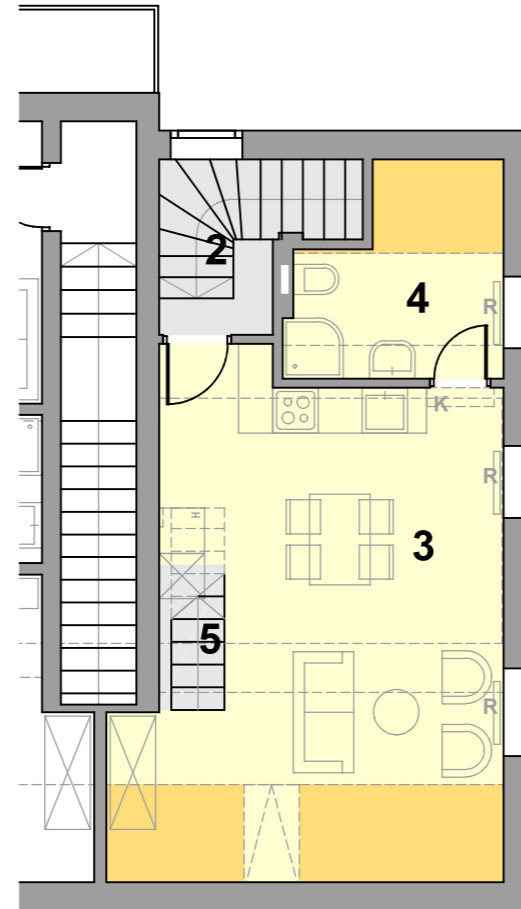
Mansarda M 1:100
