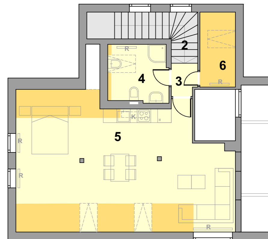
Mansarda M 1:100
